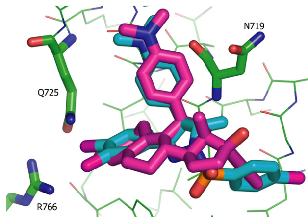
Figure 1. Progesterone receptor ligand binding domain overlay of mifepristone (magenta) with pyrazoline 7b (cyan) docked into the PR antagonist homology model.
